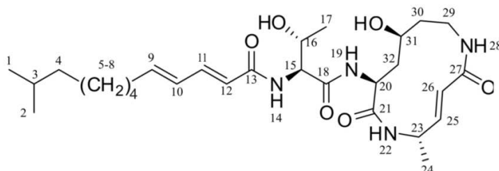
Figure 19: Structure of CepI with atom labeling.
