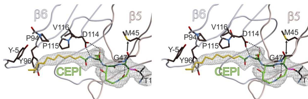
Figure 22: Stereo view of the 2F_o-F_c omit electron density map (grey mesh, 1\sigma ) of CepI in complex with the proteasomal ChTL active site. Hydrogen bonds are indicated by dashed lines, whereas the arrow underlines the accurate fitting of the P1 methyl moiety into the binding pocket without displacing Met-45 out of its original state. CepI is able to occupy the oxyanion hole formed by Gly-47N via its intracyclic peptide carbonyl moiety. Due to the rigidity of their fatty acid tails and the alignment by Asp-114, the termini of the inhibitors point towards a hydrophobic patch formed by the \beta_6 subunit. The increased hydrophobic surface of CepI compared to GlbA enhances the van-der-Waals interactions with this groove and are thus responsible for the improved binding properties of CepI. Figure adopted from Stein et al. [107] .
