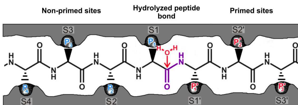
Figure 3: Schematic substrate binding channel of the active proteasomal \beta -subunits. The hydrolyzed peptide bond (violet) is initially activated by Thr-1 to form an acyl-enzyme intermediate, which in turn is attacked by an electrophilic water molecule. Adapted from Stein, M. [44] .
