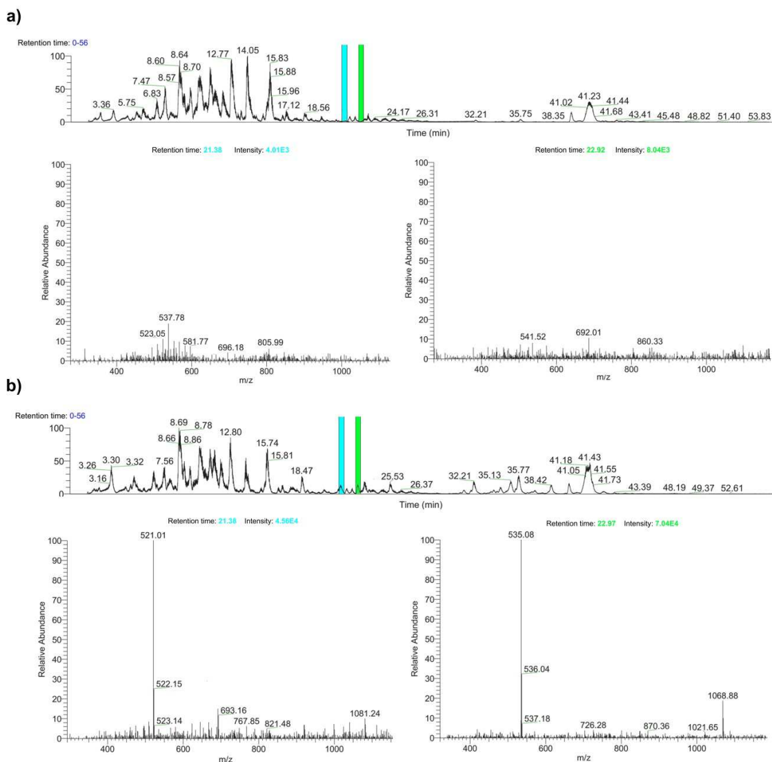
Figure 17: Mass spectrometrical analyses of P. luminescens cultures. a) Under normal growth conditions, inhibitor secretion can be detected neither by the NMR assay nor by the downstream accumulation and LC-MS analysis. b) After the induction by a suitable environmental stimulus, Photorhabdus starts to dramatically change its spectrum of secondary metabolites. Whereas the range between 0 and 20 min stays unaltered in the chromatogram, a whole array of additional substances can be visualized in the area between 20 and 40 min retention time. Among these, the highly potent proteasome inhibitors are also produced in trace amounts (blue and green interval corresponding to the masses of 521 and 535 g/mol). Even by LC-MS analysis, the compounds can only be visualized after their enrichment by the solid resin and silica column purification step, whereas the NMR assay is able to already detect them in the highly heterogeneous culture broth. Figure adopted from Stein et al. [10] .
