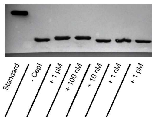
Figure 21: Reversibility experiment by western blot analysis of the \beta 5 subunit using the Pre2-(His) 6 mutant. A clear increase of the molecular mass of the active subunit is visible down to nanomolar concentrations, thereby verifying the irreversible attachment of the inhibitor. In contrast to analogous experiments with SylA, no double band occurs at the transition between the completely bound and the uninhibited state, thereby hinting at enhanced kinetic properties compared to SylA.
