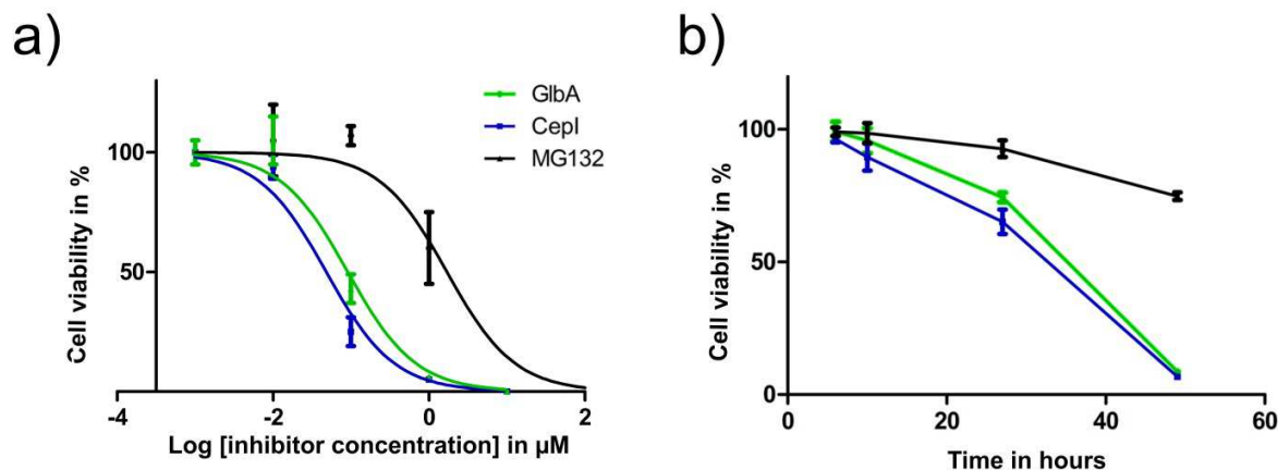
Figure 26: Cytotoxic properties of CepI and GlbA towards HeLa cancer cells in comparison with the standard aldehyde inhibitor MG132 (Z-Leu-Leu-Leu-al). a) LD 50 curves were recorded after approximately 48 h, when the inhibitors reached their maximum cytotoxicity. Both natural compounds are far more potent than MG132 with CepI being even slightly stronger than GlbA. b) The kinetic evaluation of the inhibitors was performed at final inhibitor concentrations of 1 μM. Whereas MG132 almost does not have any effect on lethality in accordance with the LD 50 measurements, the syrbactin inhibitors quantitatively kill the cells within 48 h. Again, CepI is slightly more efficient than GlbA, thus reflecting their in vitro characterization. Figure adapted from Stein et al. [107] .
