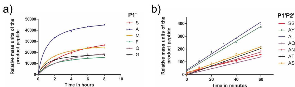
Figure 12: Kinetic measurements of substrates. The digestion progress was evaluated by LC-MS analysis. Due to the semi-quantitative character of the technique, the produced N-terminal peptide was used as a standard. a) Mutagenesis of the first primed site (P1') has a massive impact on substrate turnover. Especially small amino acids like alanine are favored. Bulky side chains as in methionine, phenylalanine or glutamine lead to a plentitude of side products as they change the proteolytic frame. The final concentrations of the detected N-terminal peptides differ considerable due to these side reactions that yield alternative fragments b) Alteration of the P2' residue also influences the kinetics, but has no effect on the regioselectivity of the cleavage. Therefore, only the initial turnover rates were monitored. The experiment clearly shows that P1' has a greater influence on the reaction than P2'. However, also the latter has a direct and substantial impact on cleavage kinetics.
