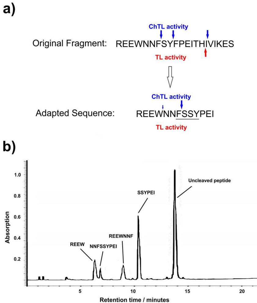
Figure 10: Peptide digestion analyses. a) The peptide was shortened compared to the original murine fragment and its sequence altered (region underlined) to increase subunit specificity. Blue and red arrows indicate proteolytic cleavage sites of the proteasomal ChTL and TL activities, respectively. b) Digestion experiments were evaluated by HPLC analyses and quantified by integration of the educt and product peaks. Peptides were identified by ESI-MS measurements. The main hydrolysis site is located after phenylalanine, whereas cleavage after tryptophan occurs only to a minor proportion of approximately 5%.
