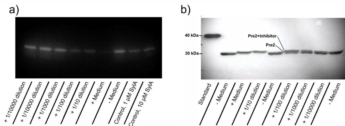
Figure 13: Orthogonal gel assays. a) Native gel with fluorescent dye development. Increasing concentrations of SyIA suppresses fluorescence. Comparison with standardized concentrations reveals that the medium contains SyIA in the micromolar range. b) Gel shift assay in denaturing SDS-PAGE using a Pre2-(His) 6 mutant. The \beta 5 subunit is selectively stained in a western blot by (His) 6 -antibodies. The gel shift confirms the covalent attachment of SyIA to the \beta 5 subunit and the extent of the shift hints at an inhibitor size of approximately 0.5 kDa.
