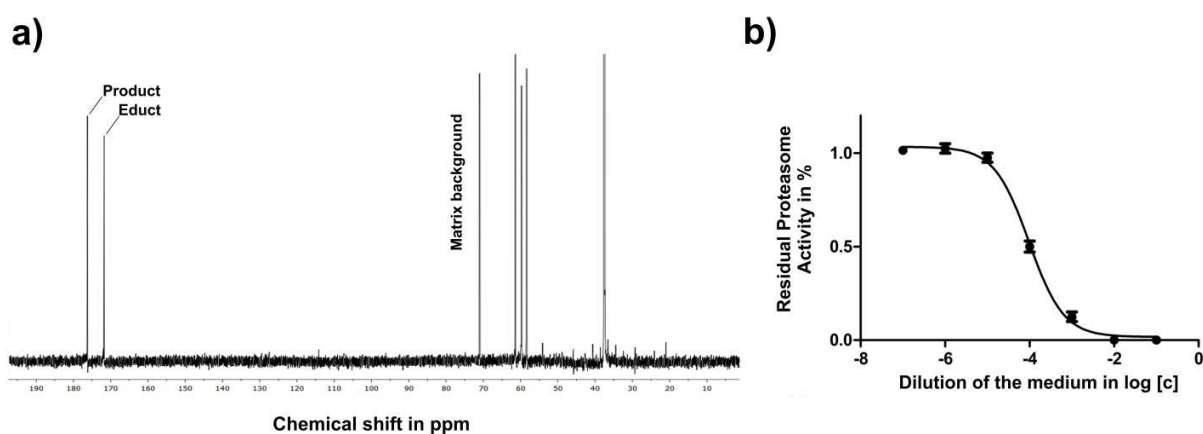
Figure 14: Analysis of P. syringae extracts by the NMR assay. a) Full ^{13}\text{C} -NMR spectrum of an exemplary digestion. The signal-to-noise ratio of the product and educt peaks (extreme left) is very high and no interference occurs with components of the medium or the buffer (peaks on the right). b) The serial dilution of the medium demonstrates that the assay is able to detect even trace amount of the inhibitor in the crude matrix.
