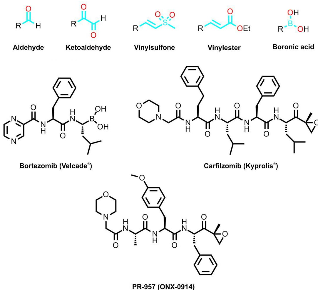
Figure 5: Described and validated electrophilic warheads of peptidic proteasome inhibitors. Bortezomib was the first prescriptive UPS inhibitor admitted by the FDA. Carfilzomib and PR-957 represent the next generation of proteasome inhibitors that rely on lead motives derived from natural secondary metabolites.
