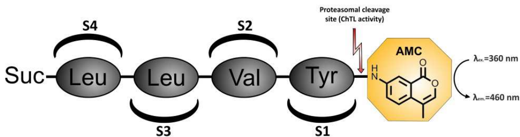
Figure 8: The most commonly applied proteasome assays use a non-natural substrate that contains a subunit-specific amino acid scaffold with a chromogenic headgroup, which is internally quenched by the attachment to the peptide. Upon cleavage by one of the proteasomal activities, the dye develops its absorptive or fluorescent properties.
