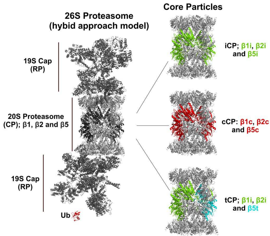
Figure 2: The 26S proteasome with an approximate molecular weight of 2.6 MDa is huge compared to the small Ub tag (red) of marked substrate proteins. Vertebrates have developed subspecies of the central catalytic machinery residing in the CP. In these particles, the proteolytic subunits are exchanged to reshuffle the cleavage activities and hence adapt to the physiological requirements. Electron microscopical model received from E. Morris [23] . Figure adapted from Stein et al. [10] .
