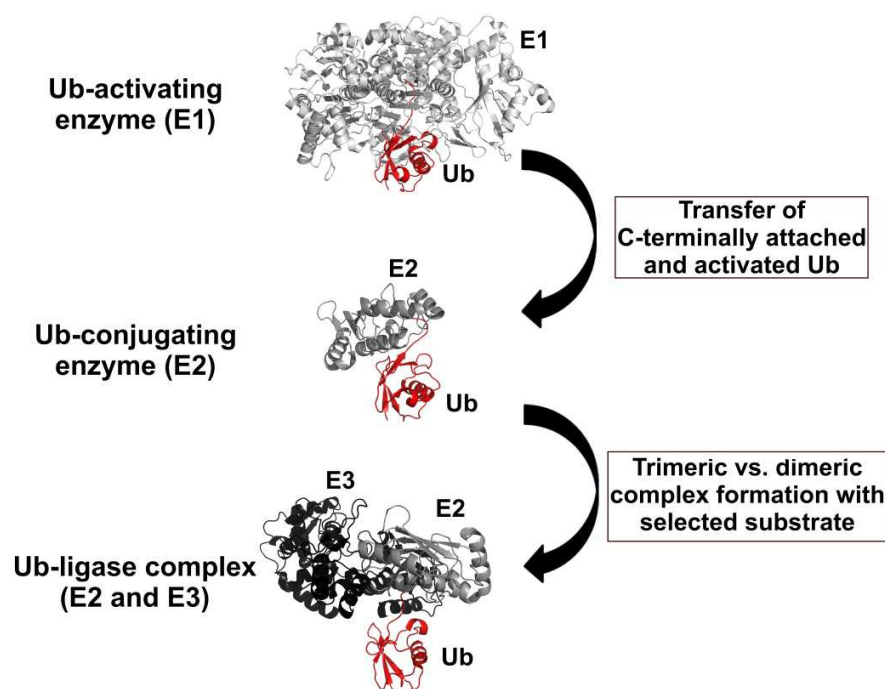
Figure 1: Ubiquitinylation involves three enzymes in a cascade-like reaction setup, which activate (E1, upper) [12] , hand over (E2) [13] and ligate (E3) [14] an Ub molecule to a growing chain attached at a suitable substrate molecule. Substrate recognition can be achieved by a E3 alone or in complex with the E2 enzyme [15] . Figure adapted from Stein et al. [10] .
