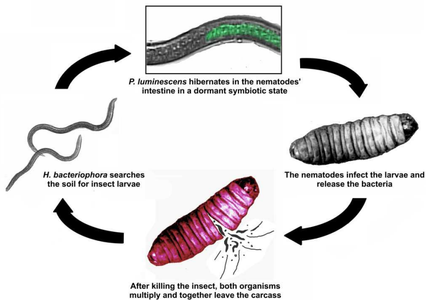
Figure 28: The bipolar life-cycle of P. luminescens is separated into a symbiotic phase during which the bacterium inactively abides in the intestine of a nematode ( H. bacteriophora ) and a pathogenic phase in the insect larva where it secretes toxic compounds as well as colourful pigments to deter other scavenging organisms. After killing the insect and multiplying in its carcass, the nematodes again swallows the bacteria and both leave the insect body to search for more prey.
