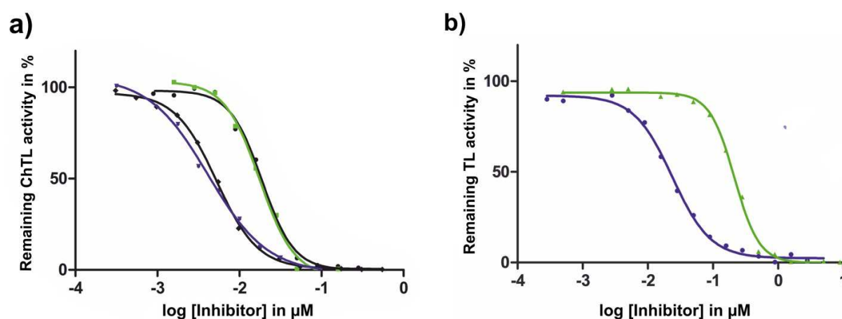
Figure 20: IC 50 curves of GlbA (green) / CepI (blue) with yeast CP. a) Evaluation of the ChTL activity shows that CepI is far more potent than GlbA, sporting IC 50 values of 4 and 19 nM, respectively. Comparison between the data produced with fluorescence and NMR (black) assays underlines the equivalency of both techniques also with regard to sensitivity. Error bars are too small to be visible. b) The inhibitory properties of both compounds can also be observed for the TL activity, despite their binding preference for the \beta 5 subunit. The IC 50 value of CepI (22 nM) is even ten times decreased compared to GlbA (214 nM).
