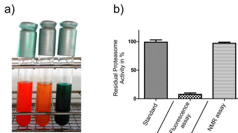
Figure 15: Quenching of conventional proteasome assays. a) Photorhabdus produces a whole variety of intensely coloured pigments, which quench the chromogenic molecules detected in these assay techniques [10] . b) The NMR assay demonstrates its superiority over these methods by avoiding the plenitude of false positive assay results.
