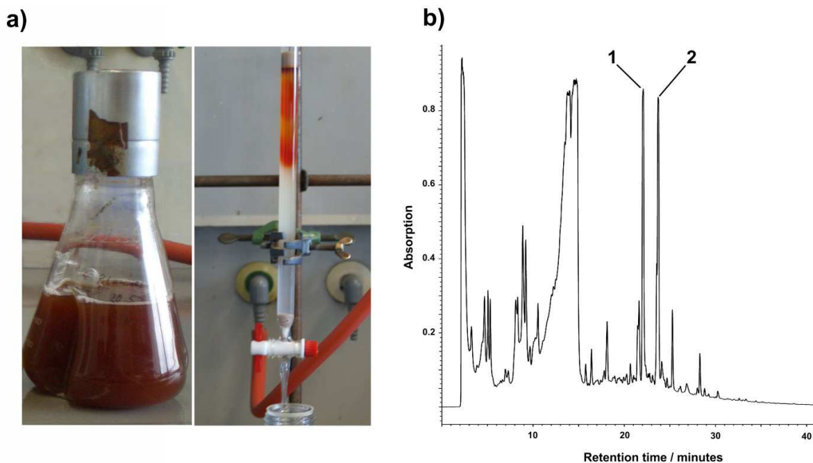
Figure 16: Column purification of the inhibiting substances. a) The growth medium of Photorhabdus occurs as non-transparent and extremely colourful suspensions. Silica column chromatography of the solid resin extract displays the variety of pigments produced by the bacterium, thereby making the NMR-based assay an indispensable tool for fraction analysis [107] . b) HPLC polishing of the active fractions. Two highly potent and lipophilic substances could be separated, which corresponded to the masses 520 and 534 g/mol. Figure adapted from Stein et al. [107] .
