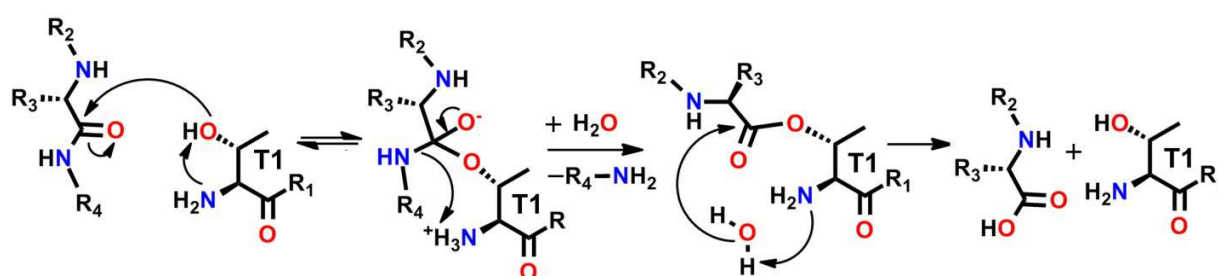
Figure 4. Catalytic peptide cleavage by the proteasomal active sites. By a nucleophilic attack of Thr-1O y on the scissile peptide bond, an acyl-enzyme intermediate is formed. Subsequently, the ester is hydrolyzed by an activated water molecule to release the N-terminal peptide fragment.
