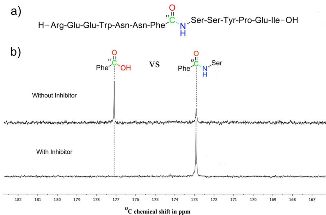
Figure 11: NMR peptide assay. a) Primary sequence of the substrate with the scissile peptide bond and the ^{13}\text{C} -label. b) NMR spectrum of substrate digestions with the uncleaved educt and the carboxylic acid product at 173 and 177 ppm, respectively (Upper). Product peak formation is suppressed upon addition of a CP-inhibiting compound (Lower). Figure adopted from Stein et al. [107] .
