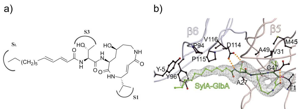
Figure 25: SylA-GlbA hybrid molecule. a) The chimera of SylA and GlbA is mostly derived from GlbA, but carries an i -propyl moiety in P1. b) Electron density map ( 1 \sigma ) of the inhibitor in complex with the proteasomal \beta 5 and \beta 6 subunits. Hydrogen bonds are indicated by dashed lines. All interactions present in the structure of GlbA can also be observed in case of the chimera. Due to the higher spatial requirements of the i -propyl moiety, M45 is dislocated to enlarge the S1 pocket [140] .
