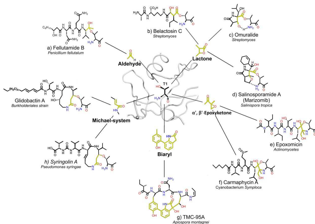
Figure 6: Natural proteasome inhibitors of the 20S proteasome. a) The linear peptide aldehyde fellutamide B and b) the \beta -lactone belactosin C were among the first identified natural proteasome inhibitors. c) Omuralide and d) salinosporamide A suppress the reactivation of the enzymatic functions by dislocating the nucleophilic water molecule via a hydroxyl and a tetrahydrofuran moiety, respectively. e-f) The bifunctional \alpha', \beta' -epoxyketone warhead of epoxomicin and carmaphycin A is exploited in the prescriptive drug carfilzomib and the immunoproteasome inhibitor PR-957. The electrophilic pharmacophore reacts both with Thr-10 y and Thr-1N to form an irreversible morpholino ring derivative. g) TMC-95A is the only non-covalent natural product inhibitor identified to date. The rigid biaryl-bridged peptide scaffold carries many decorations and chiral centers that shape the compound's three dimensional structure, thus balancing the enthalpic loss by enhanced entropic properties. h) Syringolin A and g) glidobactin A are the eponymous compounds for the group of syrbactins. The constrained 14-membered macrolactam ring contains an electrophilic Michael system that generates an irreversible ether with the catalytically active Thr-10 y . Figure adopted from Stein et al. [10] .
