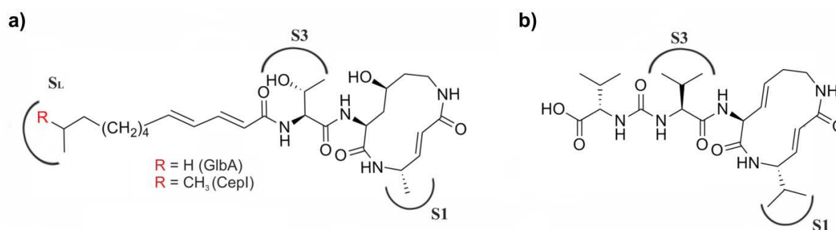
Figure 18: Structural comparison between the isolated molecules with SylA. a) GlbA and CepI share the macrolactam cycle of syrbactin compounds containing an electrophilic Michael system. Both molecules only differ in their fatty acid moiety, which carries a branched terminus in the case of CepI, whereas it is linear in GlbA. b) In contrast to the molecules produced by Photorhabdus , SylA displays a highly hydrophilic carboxylic acid tail, which is connected to the macrolactam moiety by a urea link. Eventually, its decoration pattern slightly differs, especially with regard to the moieties that interact with the S1 and S3 pockets. Figure adopted from Stein et al. [107] .
