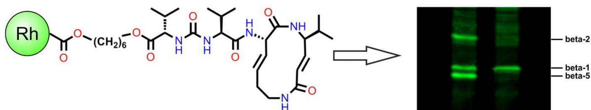
Figure 9: Site-directed-affinity-probe (SSAP) methods exploit the specific interaction of an inhibitor that is covalently linked to a chromophor. In this case, SylA is coupled to rhodamine via an alkyle linker moiety. Upon binding to the active proteasomal subunits, these can be visualized by SDS-gel separation and subsequent fluorescence detection (left lane). However, if an inhibiting sample is added to the proteasome before staining, blocked subunits cannot be tagged with the dye and in turn vanish on the developed gel (right lane). Figure adapted from Stein et al. [10] .
