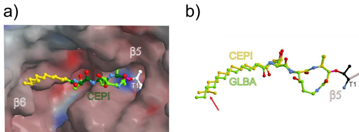
Figure 23: a) Surface representation of CepI in the binding channel formed by \beta 5 and \beta 6 . Surface colours indicate the positive (red) and negative (blue) electrostatic potential contoured from -30\text{kT/e} to +30\text{kT/e} . The aliphatic tail follows the curvature formed by \beta 6 and tightly interacts with the hydrophobic patch at its distal end. b) Superposition of GlbA and CepI derived from their respective complex crystal structures to the yeast CP. The structures perfectly match with the exception of the additional methyl moiety in CepI, which is indicated by a red arrow. Figure adopted from Stein et al. [107] .
